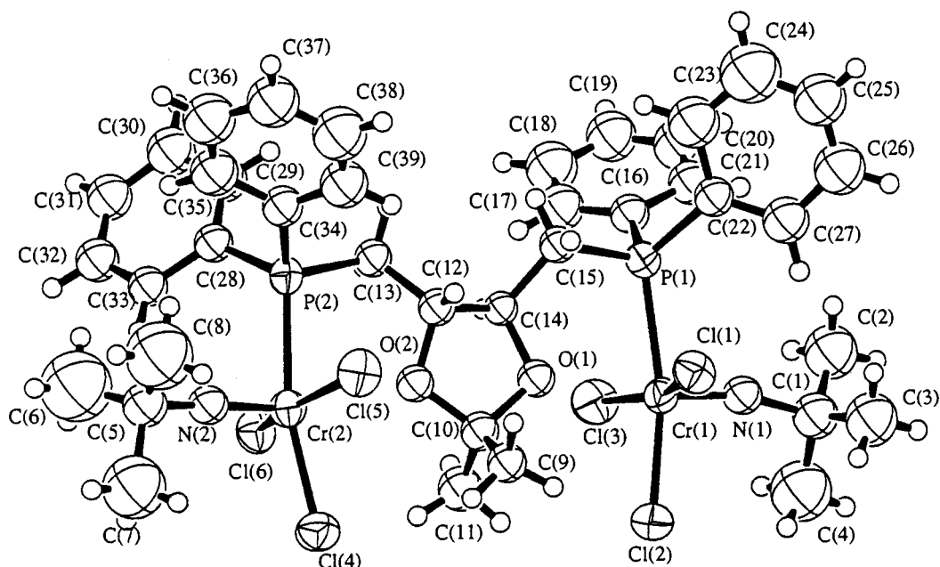
Fig. 2 Perspective view of [\{\text{Cr}(\text{NBu})\text{Cl}_3\}_2\{\mu\text{-(S,S)-diop}\}] 4
